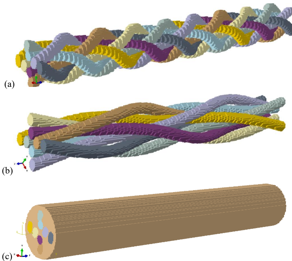
Figure 4 Virtual beams voxel-FE models : (a) '9 variant' model 8 yarns architecture, (b) '4.5 variant' model 8 yarns architecture, (c) complete beam with glass/epoxy 9ppc yarns and epoxy matrix.
