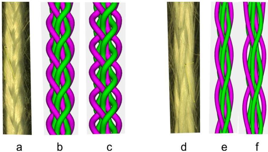
Figure 2 Investigated braids for beams a) ad d) produced structures with 9ppc and 4.5ppc, b) and d) - modelled geometry in correct scale, but with small yarn intersection regions, c) and f) slightly expanded geometry, free of intersections
