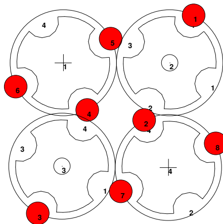
Figure 1 Configuration of the braiding machine for the braided beam production
