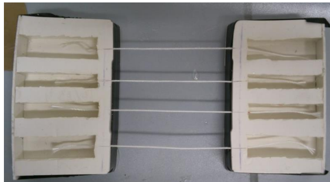
Figure 5. Embedding the samples in epoxy blocks at the both ends for avoiding the influence of the clamp damages over the testing results
