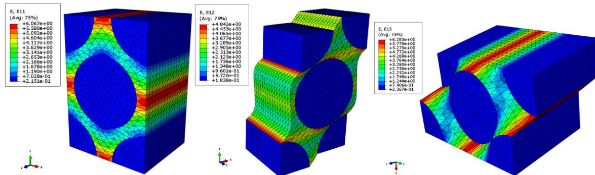
Figure 3 Deformed REV for the microscopic homogenization of yarns with boundary conditions sets: (left) 11, (center) 12 and (right) 13.
