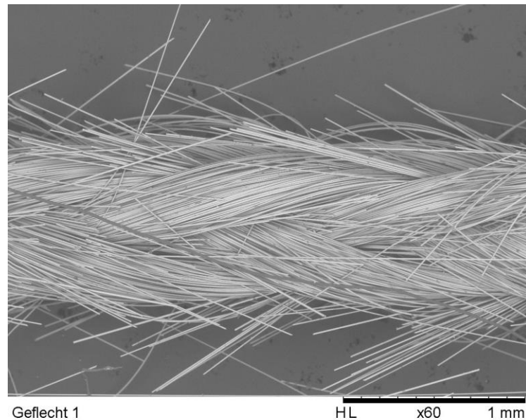
Figure 6. REM image of the dry braid, where the large amount of fiber damages are visible.
