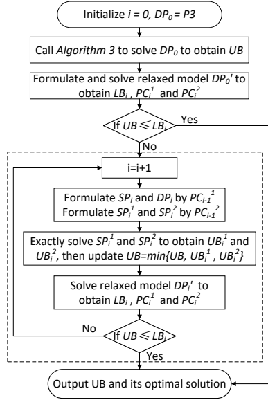
Figure 4: The framework of lifted cut-and-solve method
