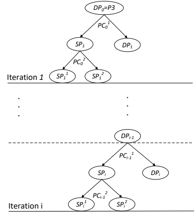
Figure 5: The search tree of lifted cut-and-solve method
